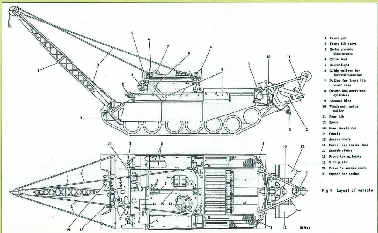
An extract from the operator's manual, showing the general arrangement of the ARV Mark 2. The front lifting jib is shown in the working position. Although carried on the vehicles it was rarely used due to the time needed to assemble the jib and its inability to slew
