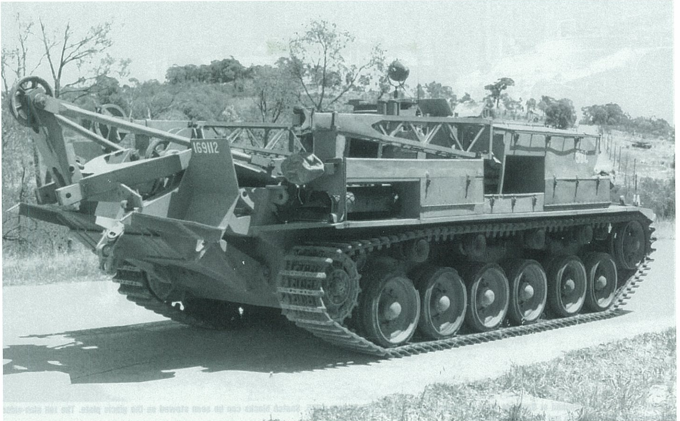
A rear view of the ARV Mark 2 with anchor spade raised in the travelling position. The rear jib can be seen as can the two sections of the lattice jib carried on top of the stowage boxes
