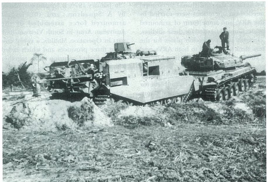
A Centurion ARV Mark 2 in South Vietnam during 1968. The anchor spade is embedded in the ground and the winch rope has been reeved into a 3 to 1 layout. A Centurion MBT has been hooked onto the front of the ARV to provide an additional anchor. The ARV has the rear deck protection plates fitted and a shield on the commander's machine gun
