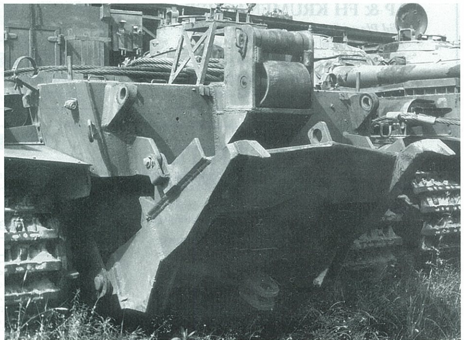
The rear anchor spade and fairlead assembly of the ARV Mark 1. The relatively light construction of the spade compared to that of the Mark 2 can be seen
